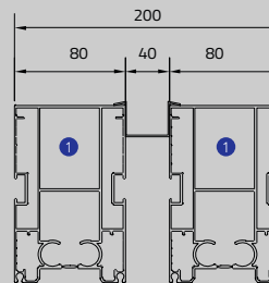
Connection Roof
