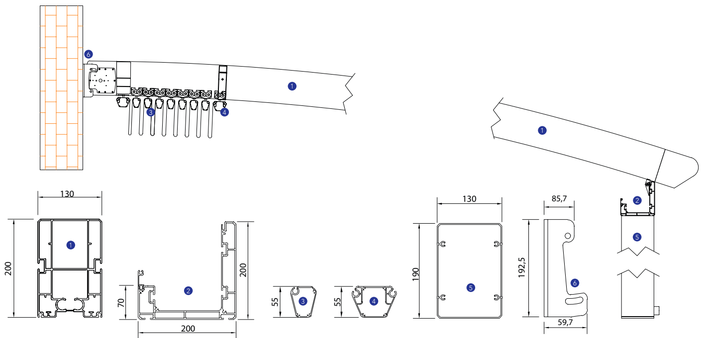
Frontal view
