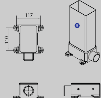
Wall application bracket
