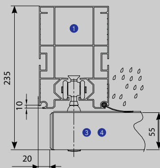
Anti-Wind profile
