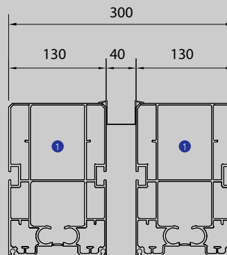
Connection roof
