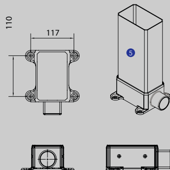
Foot
