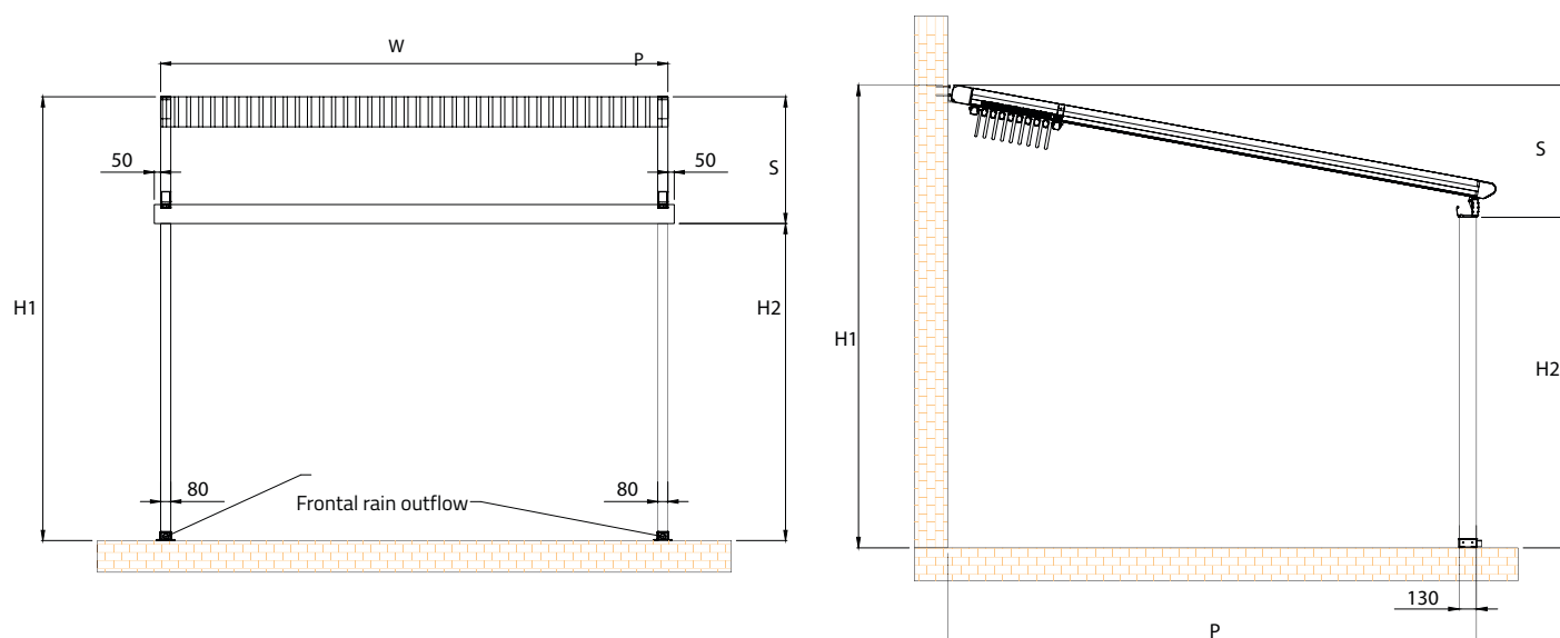
Frontal view
