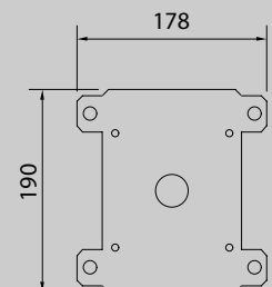
Standard foot
