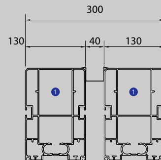
Connection roof
