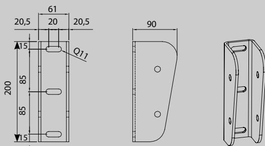
Plate for tie-rod connection
