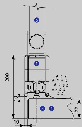
Anti-Wind profile
