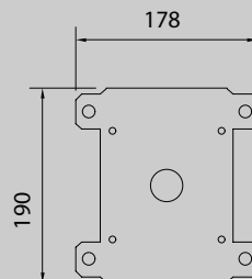
Standard foot
