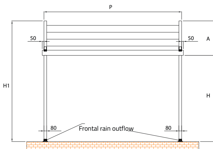
Frontal view
