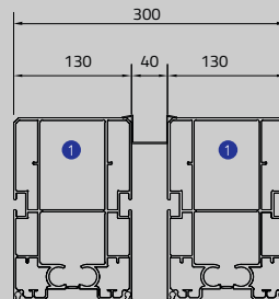
Connection Roof
