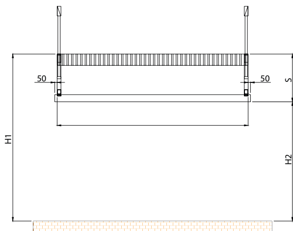
Frontal view
