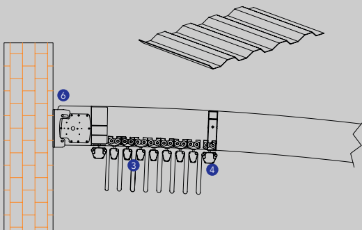
Roof detail
