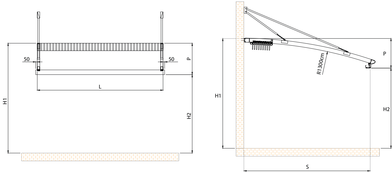
Frontal view
