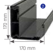
Extruded Frontal Gutter (Water-drain)
