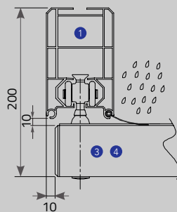
Anti -Wind profile
