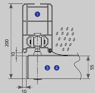
Anti-Wind Profile
