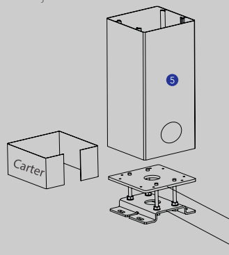
Adjustable foot
