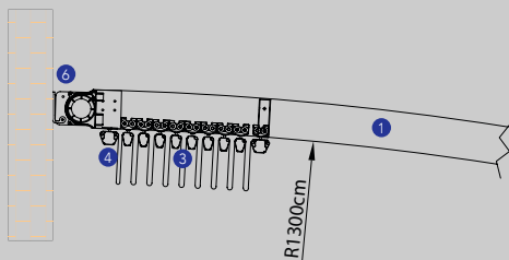
Roof for cassette
