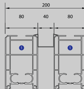
Connection roof
