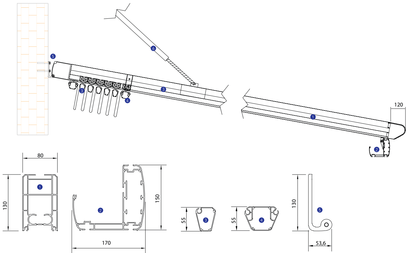
Side view
