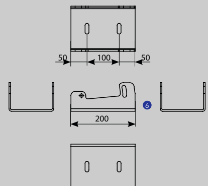
Wall application bracket
