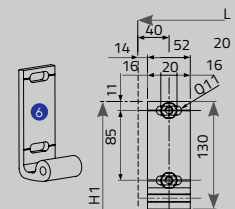
Wall Application Bracket
