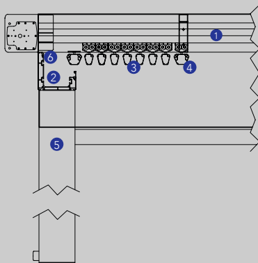
Roof Detail
