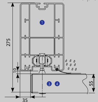
Anti -Wind profile
