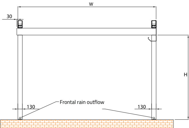
Frontal view
