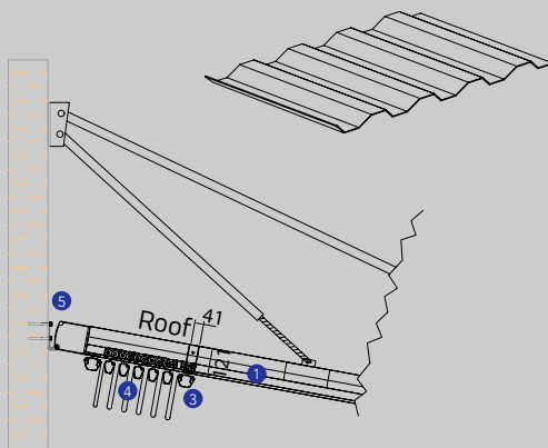
Roof detail
