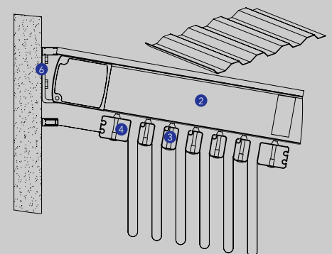
Wall Application Bracket
