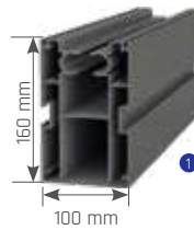
Rails
