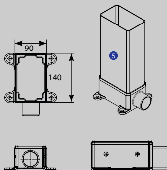
Foot
