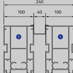
Connection Roof
