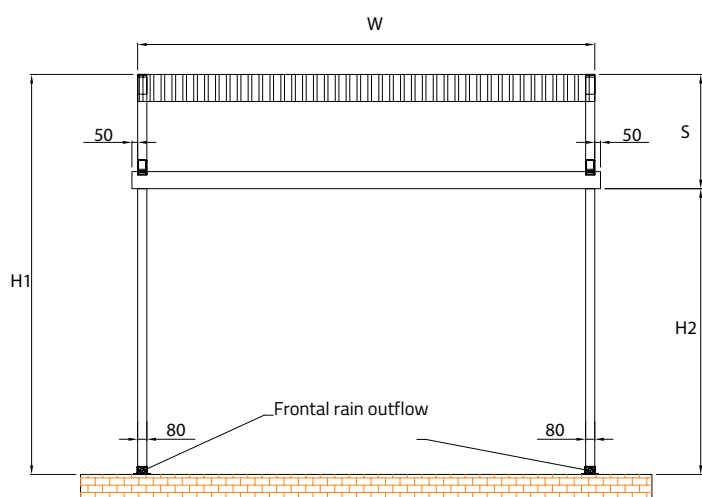
Frontal view
