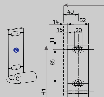
Wall Application Bracket
