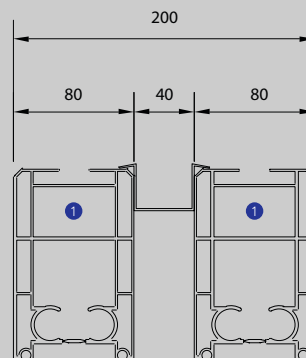
Connection roof
