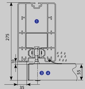
Anti-Wind profile
