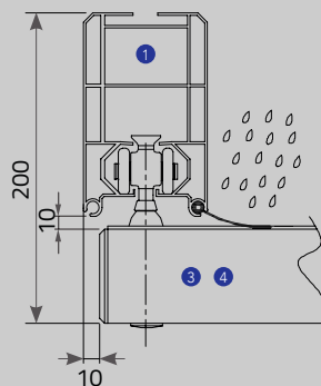
Anti-Wind Profile
