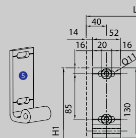
Wall application bracket
