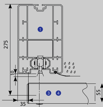
Anti-Wind profile
