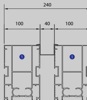
Connection roof
