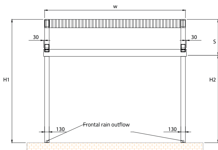
Frontal view
