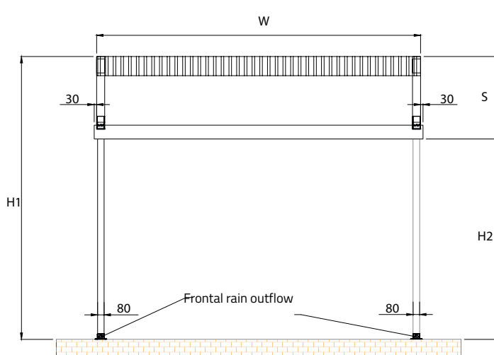
Frontal view
