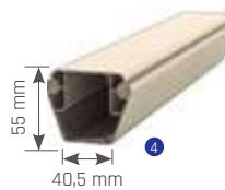
Fabric Profile
