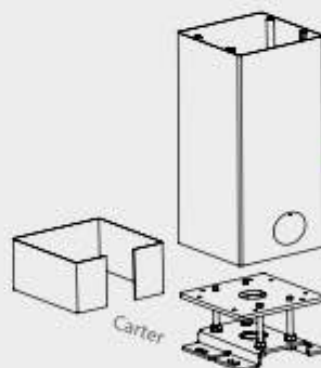
Adjustable foot
